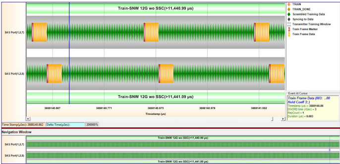
Figure 3. TX/RX Training Graphical Display
